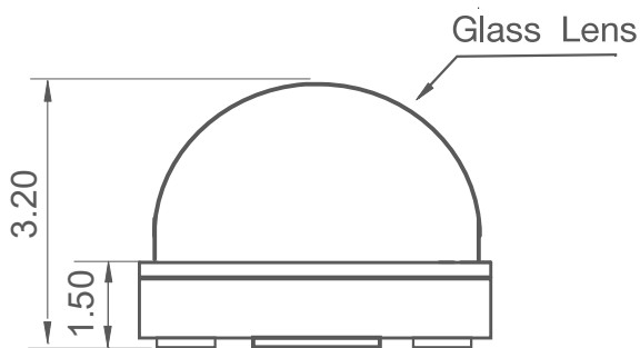
Fig.1-3 Side view 侧面视图
