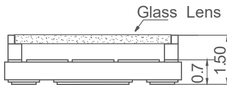
Fig.1-3 Side view 侧面视图
